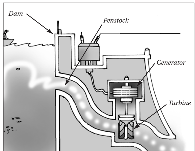
Hydroelectric Dam
